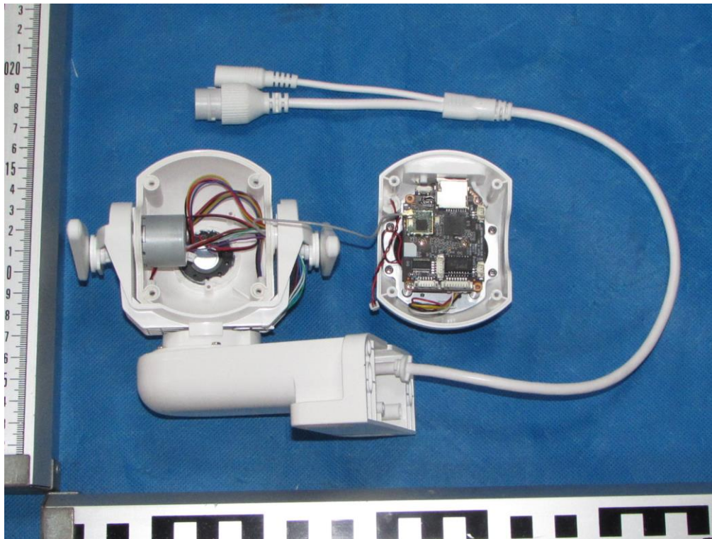
Figure 9. Internal view
