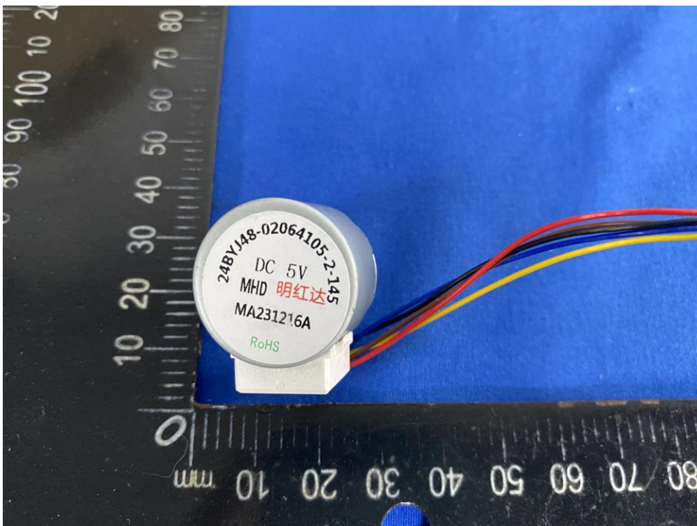
Figure 14. Stepper motor view
