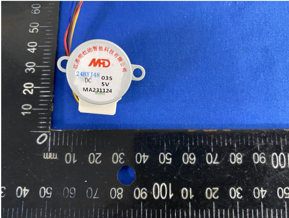
Figure 13. Stepper motor view
