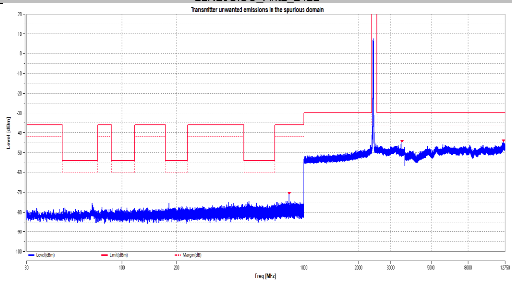
11N20SISO Ant1 2472
