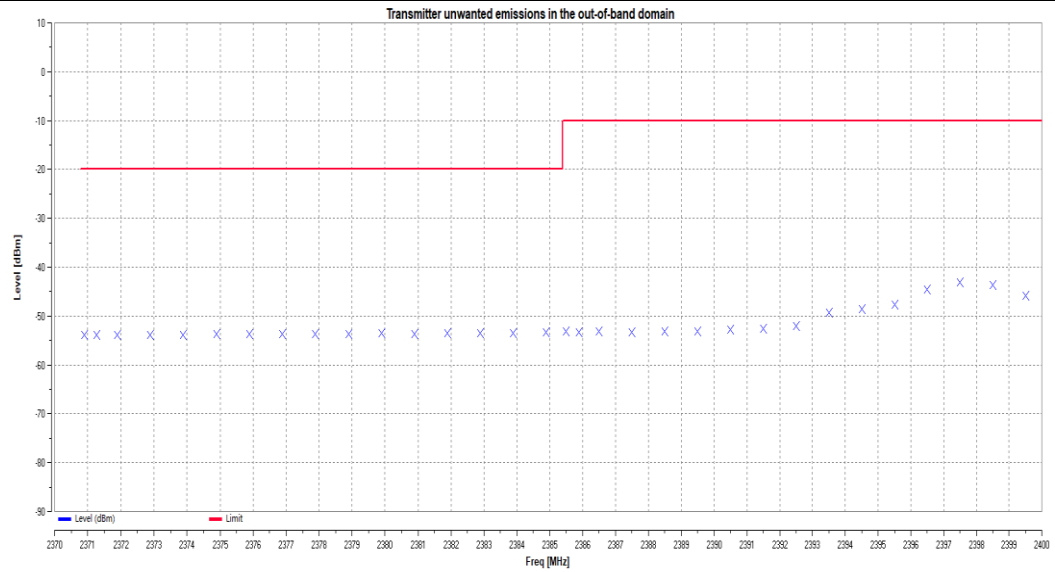
11B_Ant1_2412_2483.5MHz-2BW to 2483.5MHz+2BW
