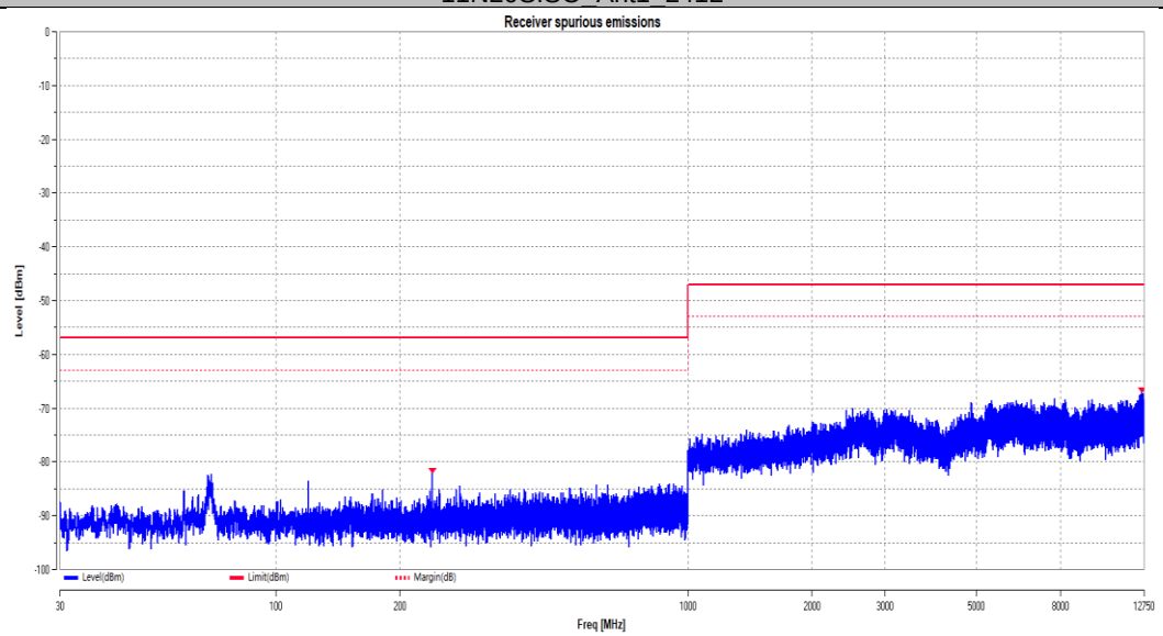
11N20SISO Ant1 2472
