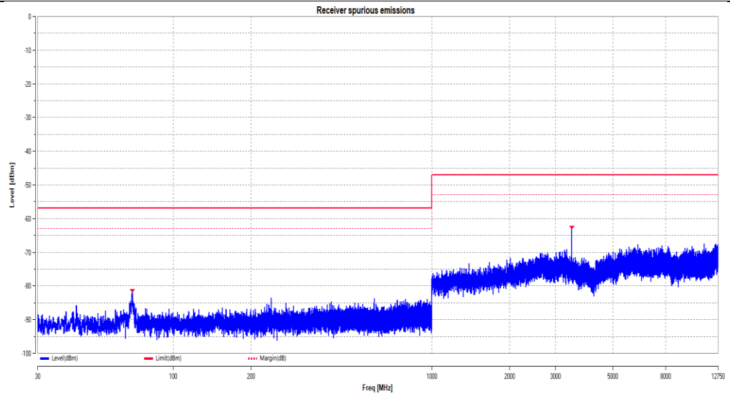
11N20SISO Ant1 2412
